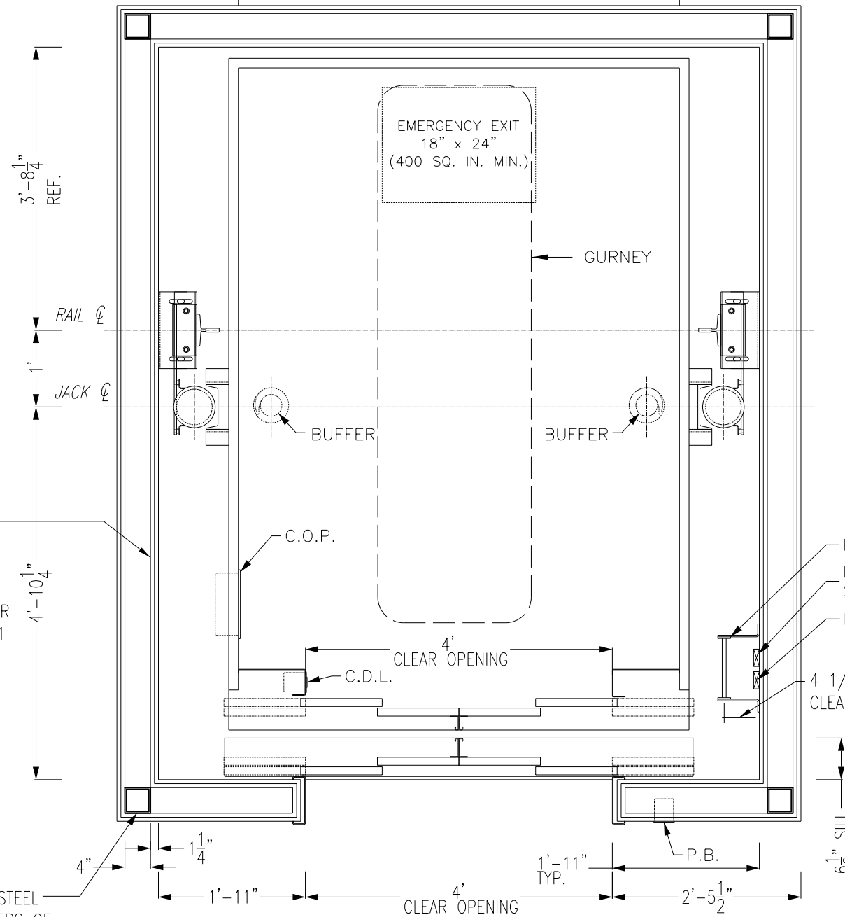
HOISTWAY PLAN
