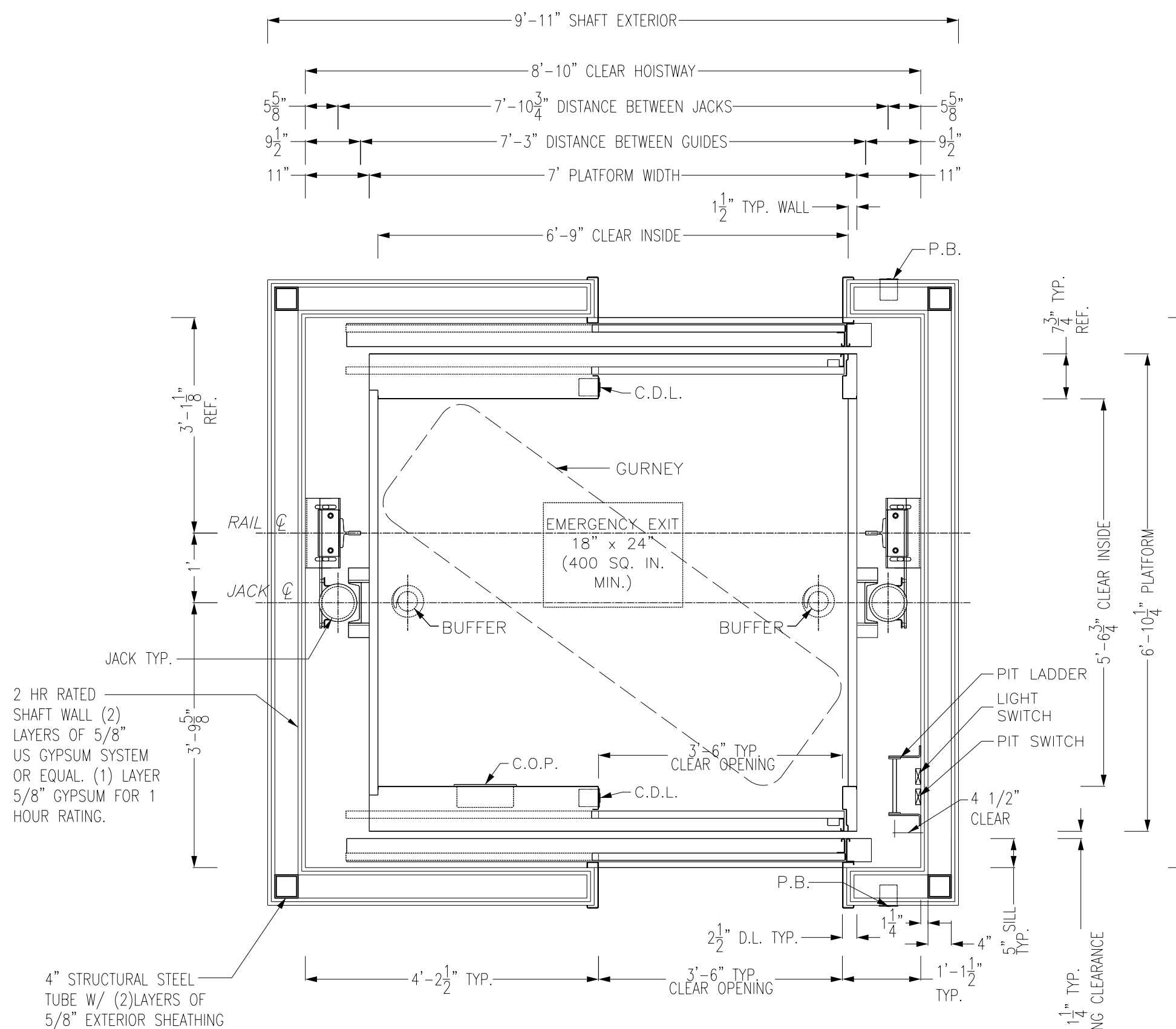
HOISTWAY PLAN
