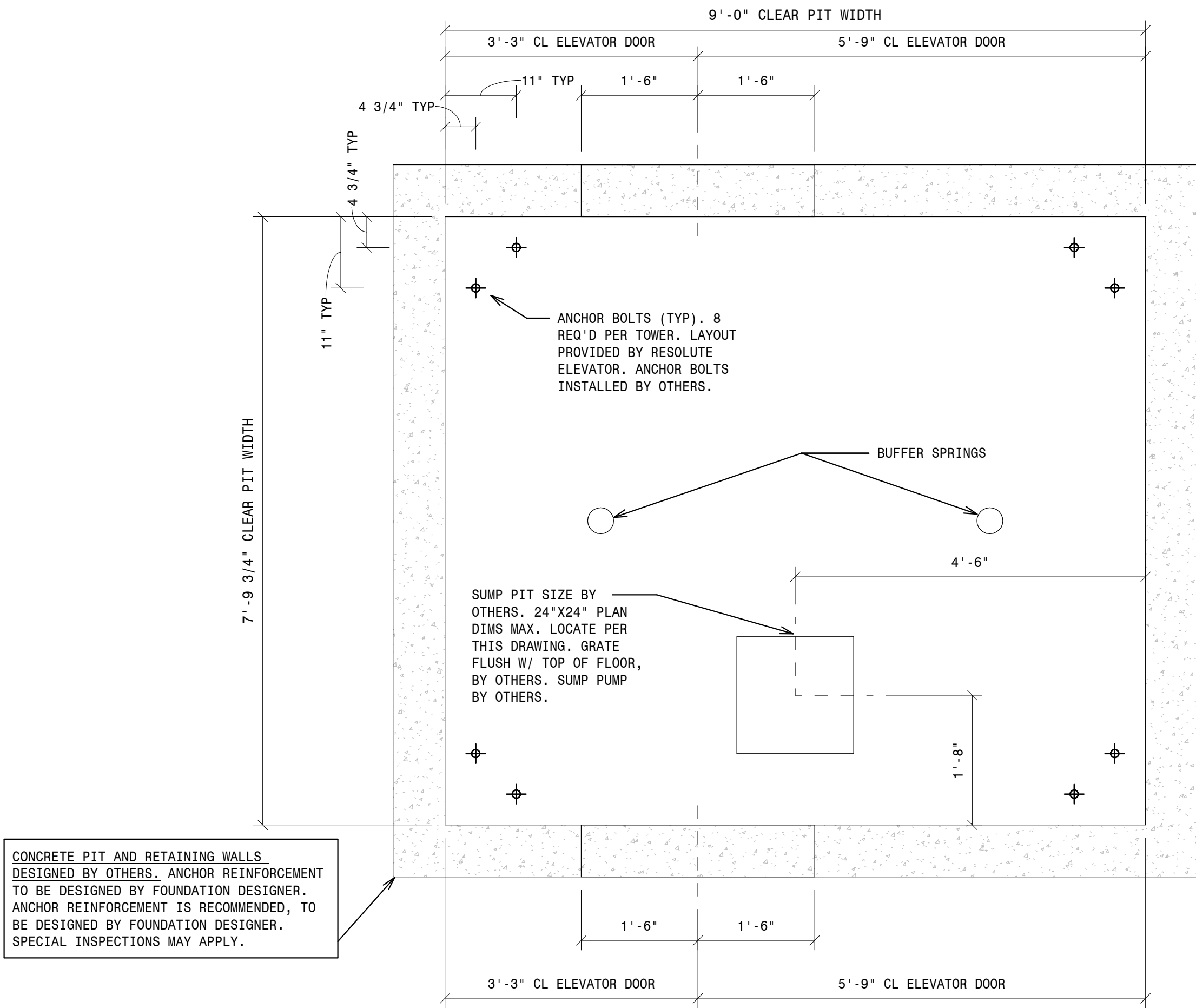
- 1 - 2100 MRL FR PIT LEFT HAND 3/4" = 1'-0"
