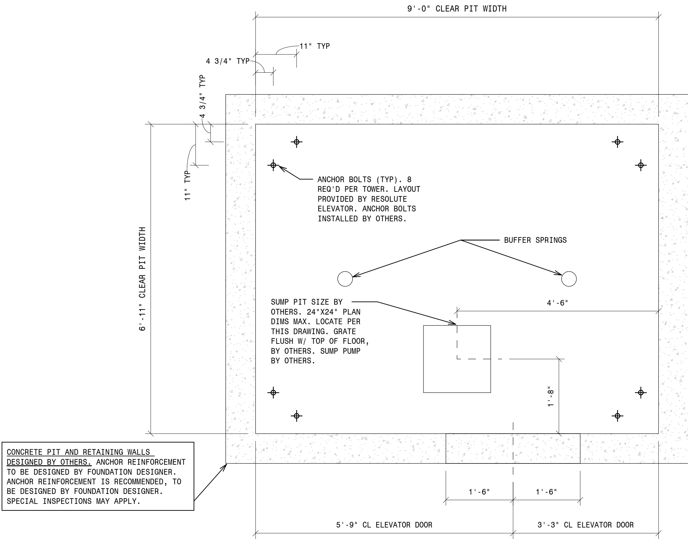
- 1 - 2100 MRL PIT RIGHT HAND 3/4" = 1'-0"
