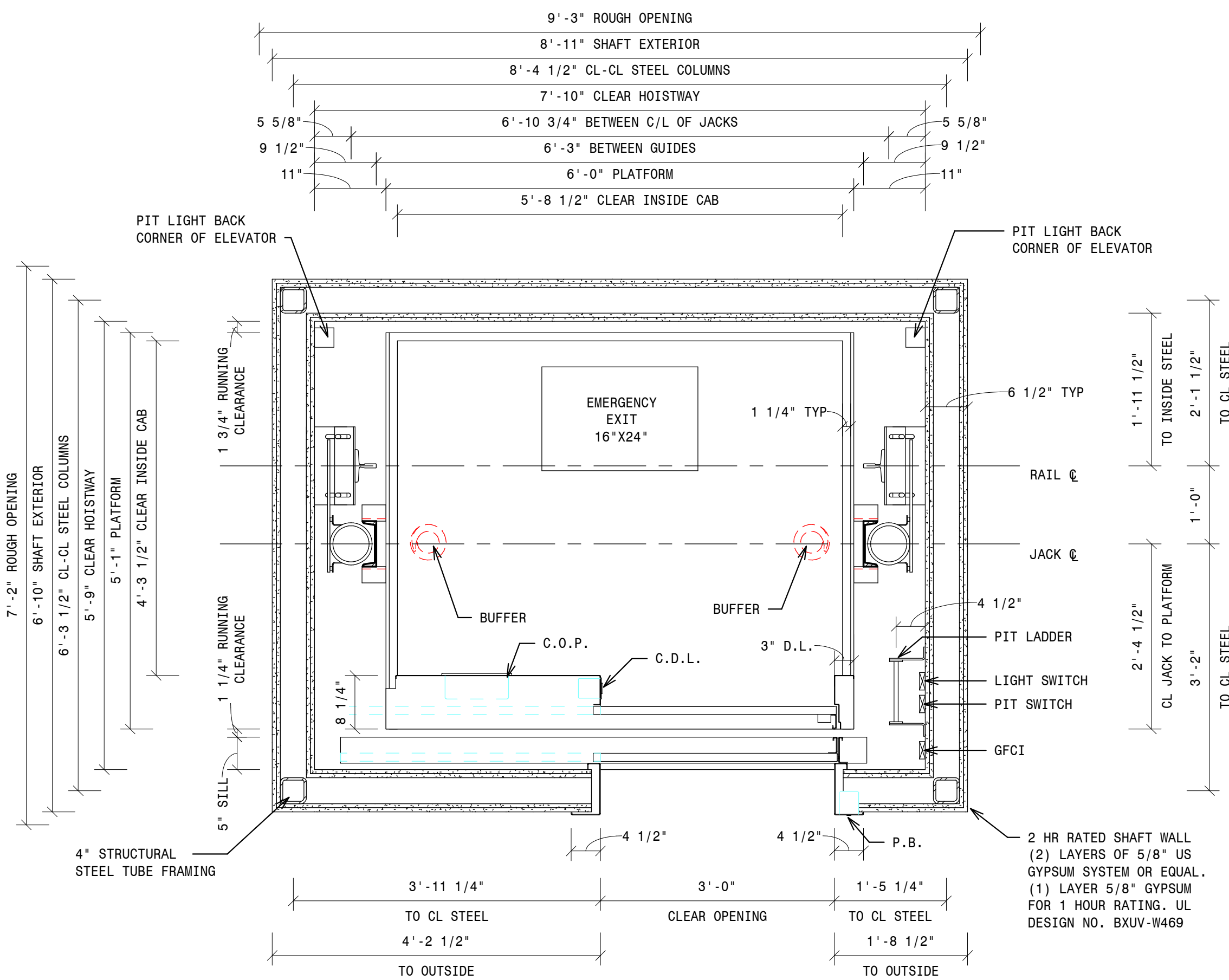
- 2 - 2100 MRL HOISTWAY RIGHT HAND 3/4" = 1'-0"
