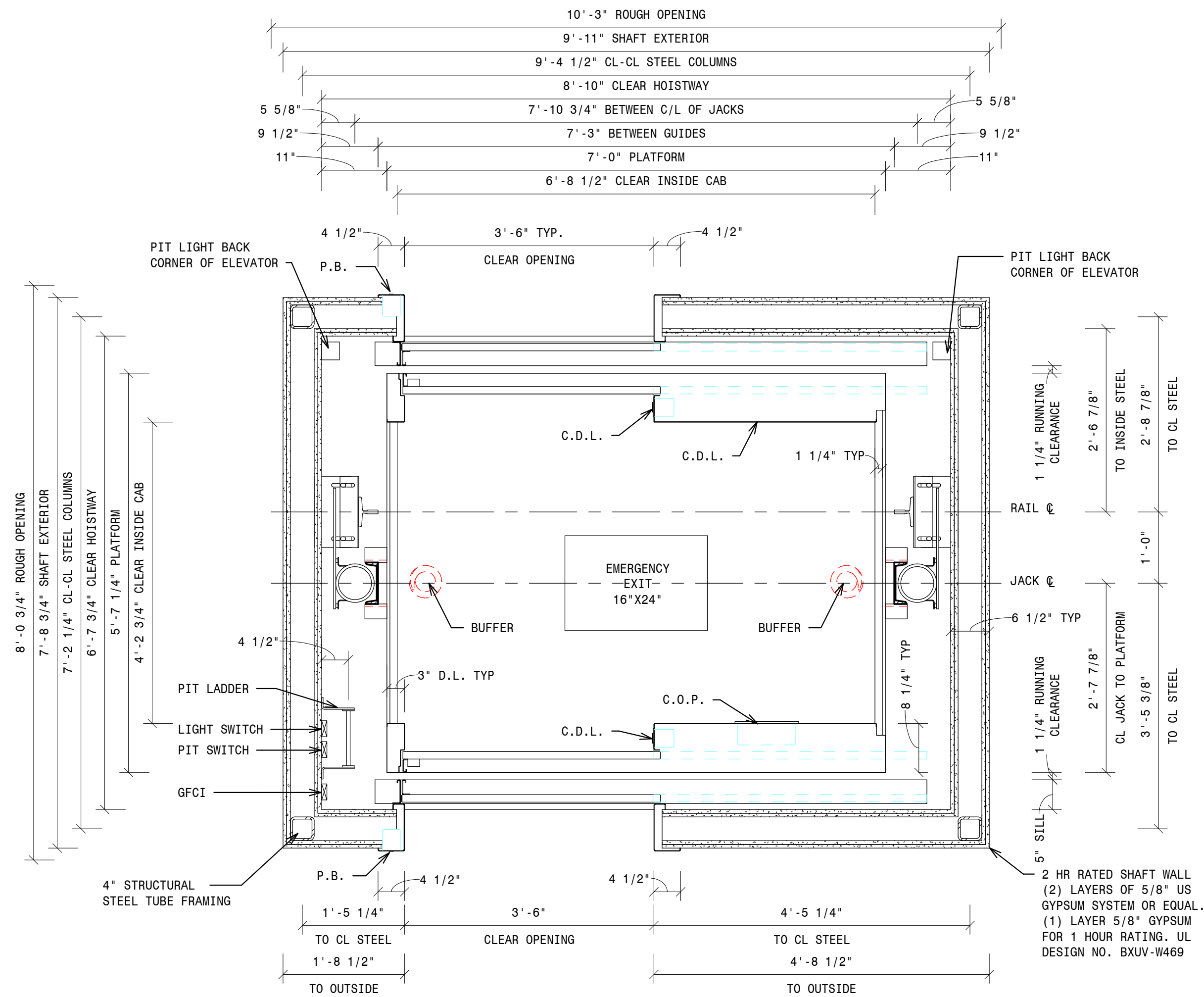
- 2 - 2500 MRL FR HOISTWAY LEFT HAND 3/4" = 1'-0"
