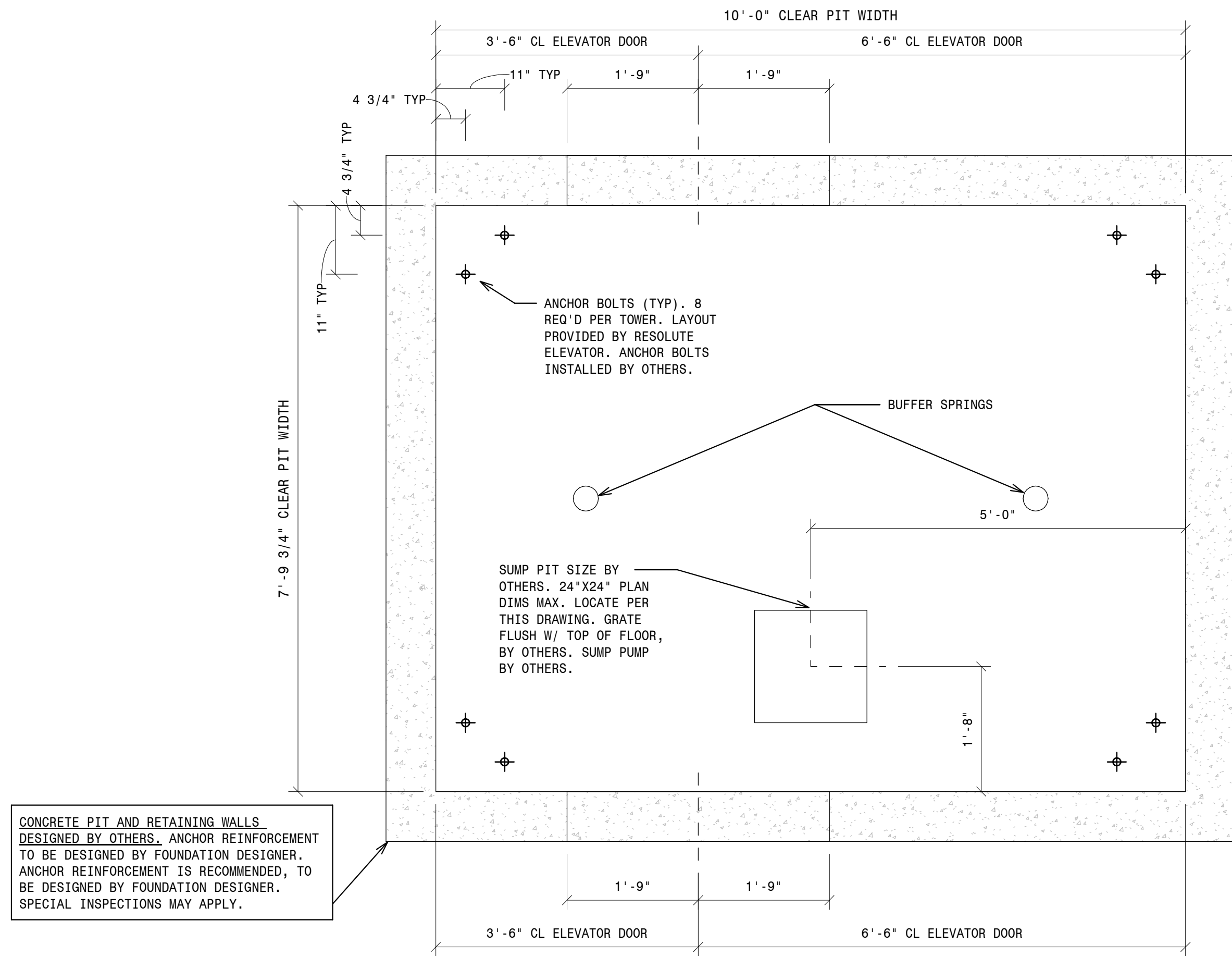
- 1 - 2500 MRL FR PIT LEFT HAND 3/4" = 1'-0"
