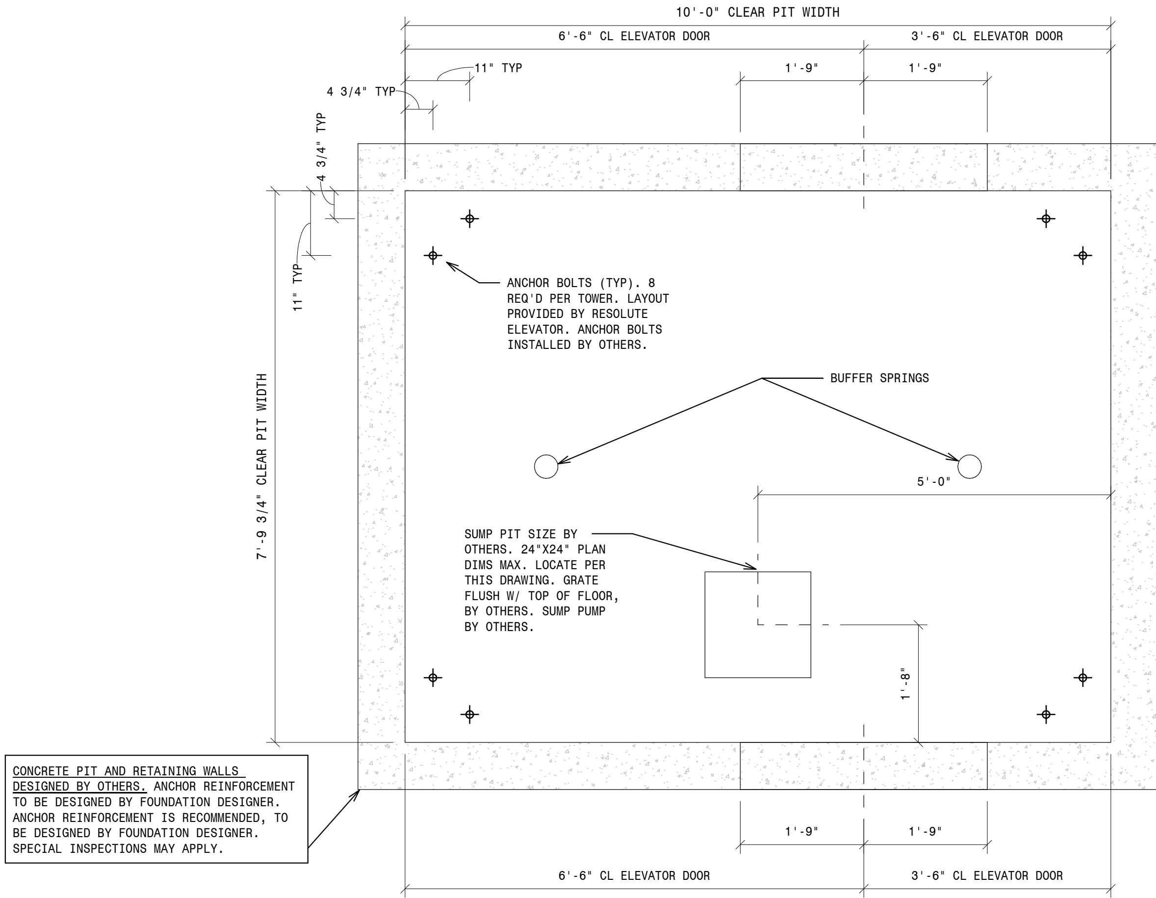
- 1 - 2500 MRL FR PIT RIGHT HAND 3/4" = 1'-0"
