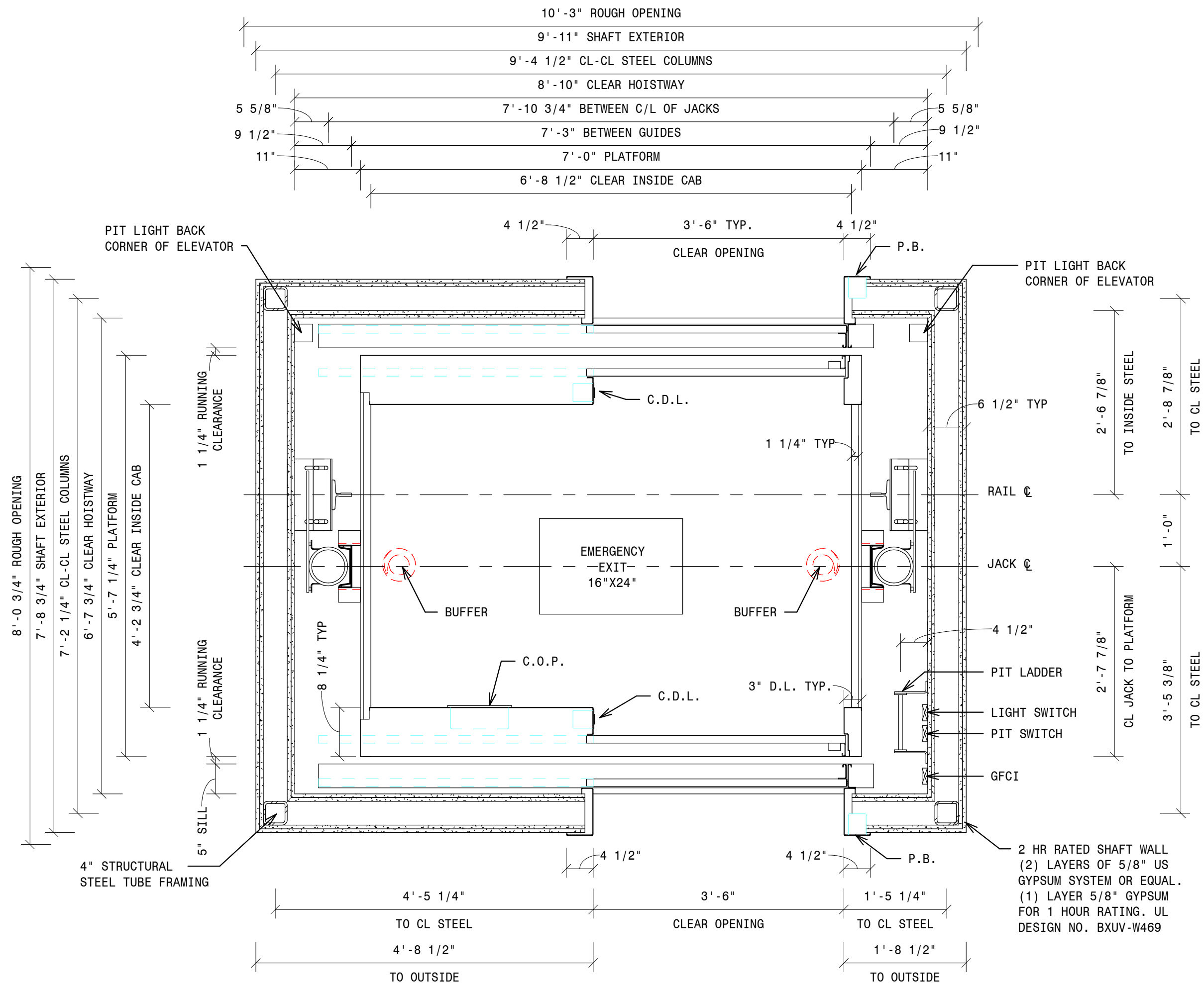
- 2 - 2500 MRL FR HOISTWAY RIGHT HAND 3/4" = 1'-0"
