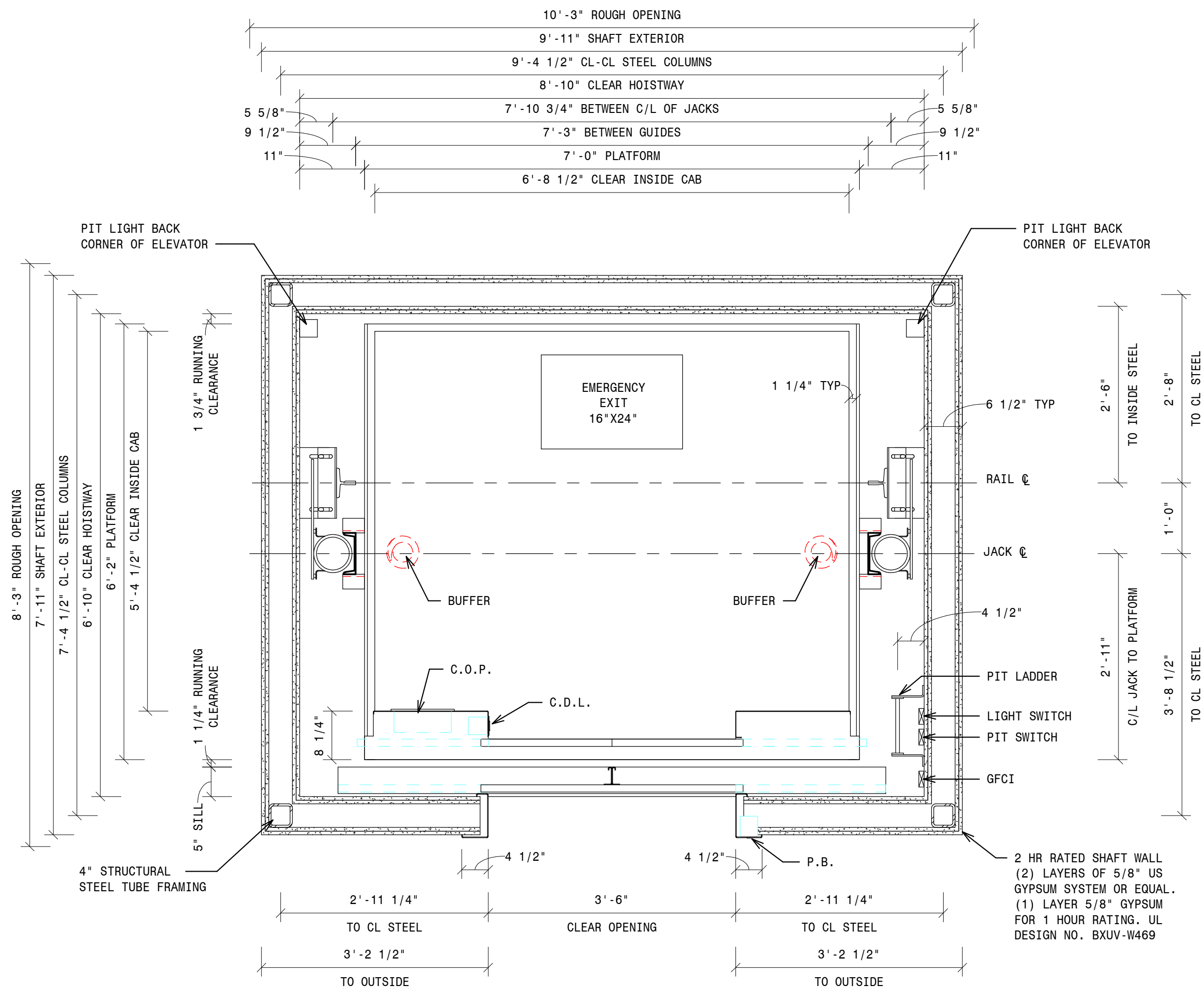
- 2 - 3500 MRL HOISTWAY CENTER 3/4" = 1'-0"
