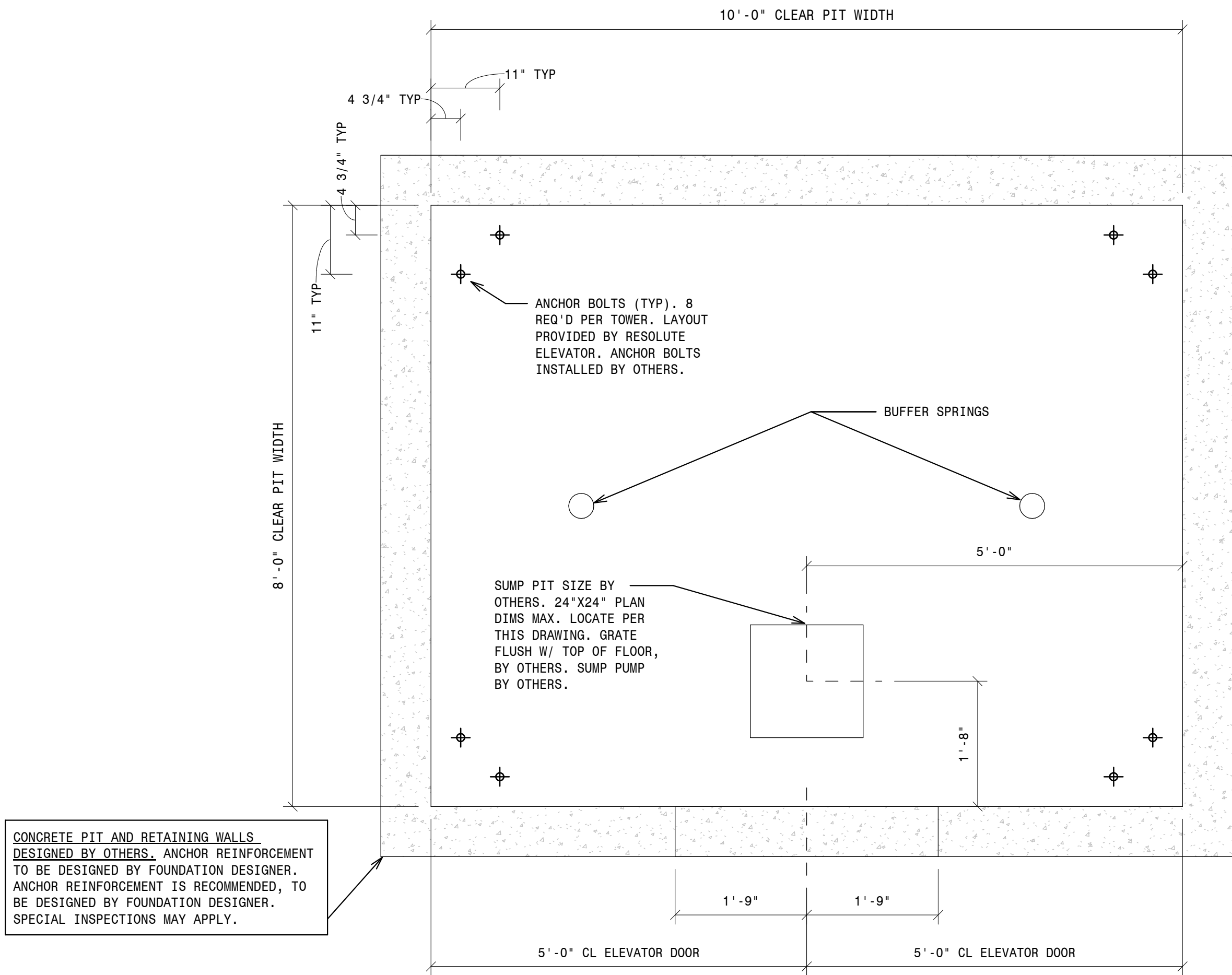
- 1 - 3500 MRL PIT CENTER 3/4" = 1'-0"
