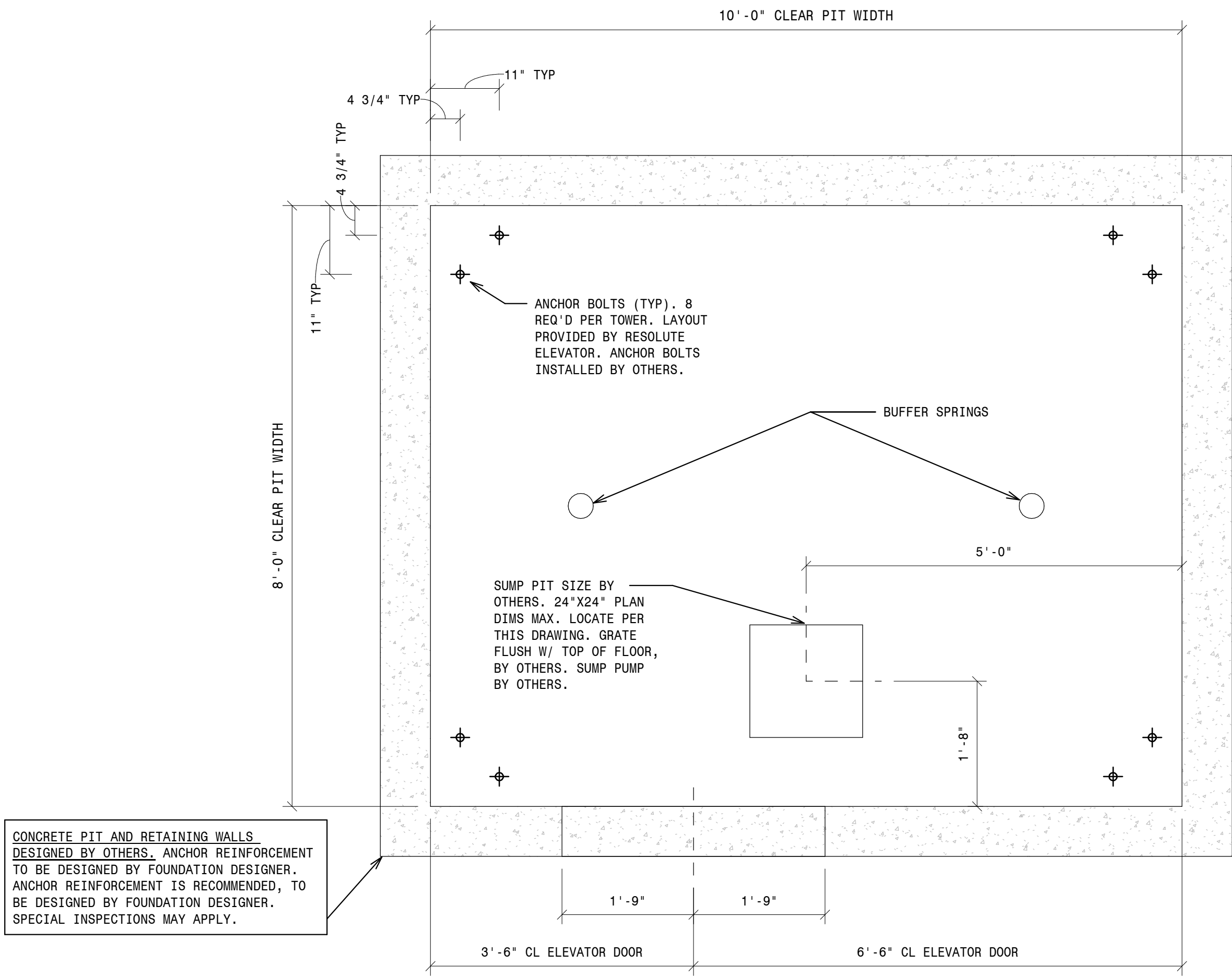
- 1 - 3500 MRL PIT LEFT HAND 3/4" = 1'-0"
