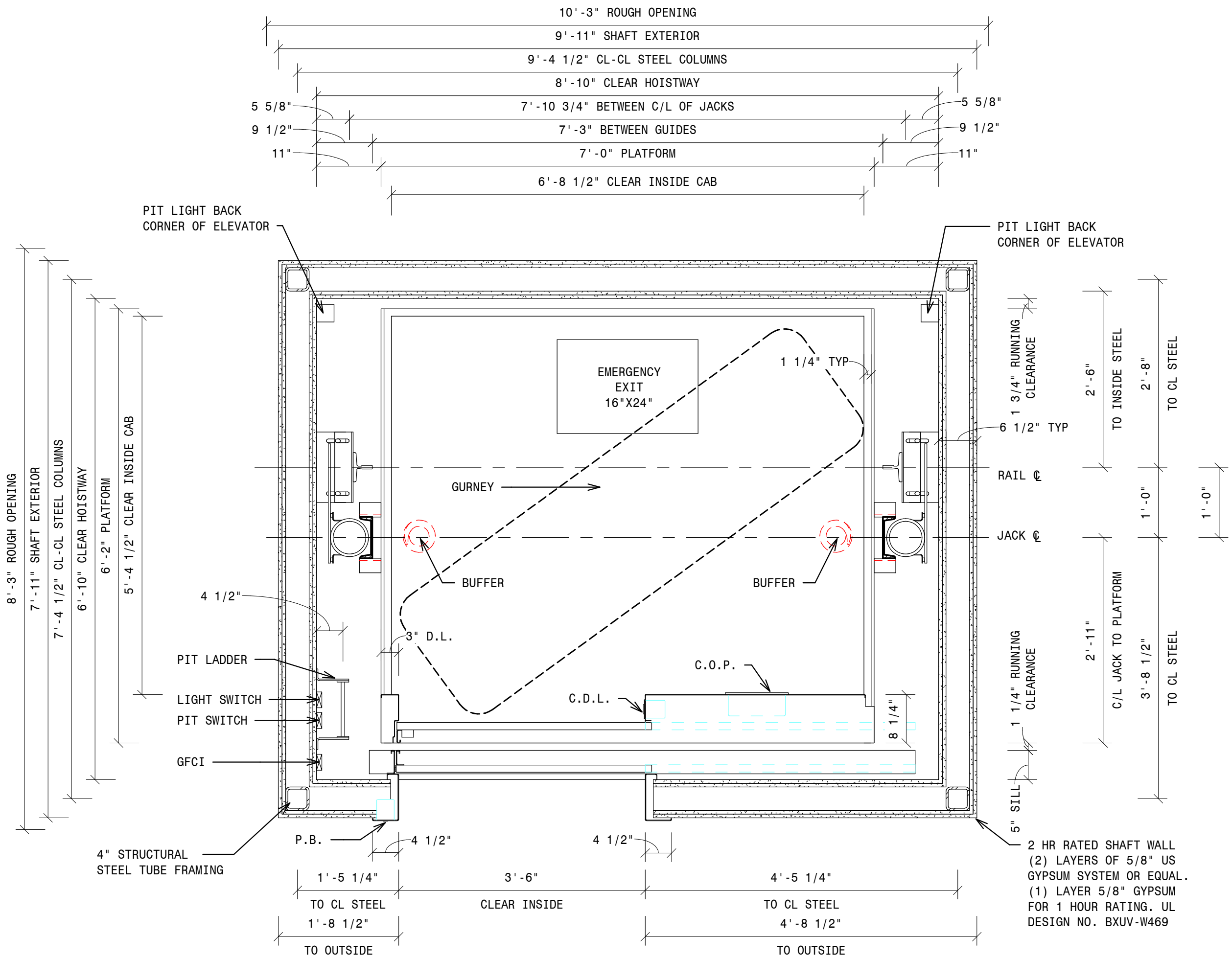
- 2 - 3500 MRL HOISTWAY LEFT HAND 3/4" = 1'-0"
