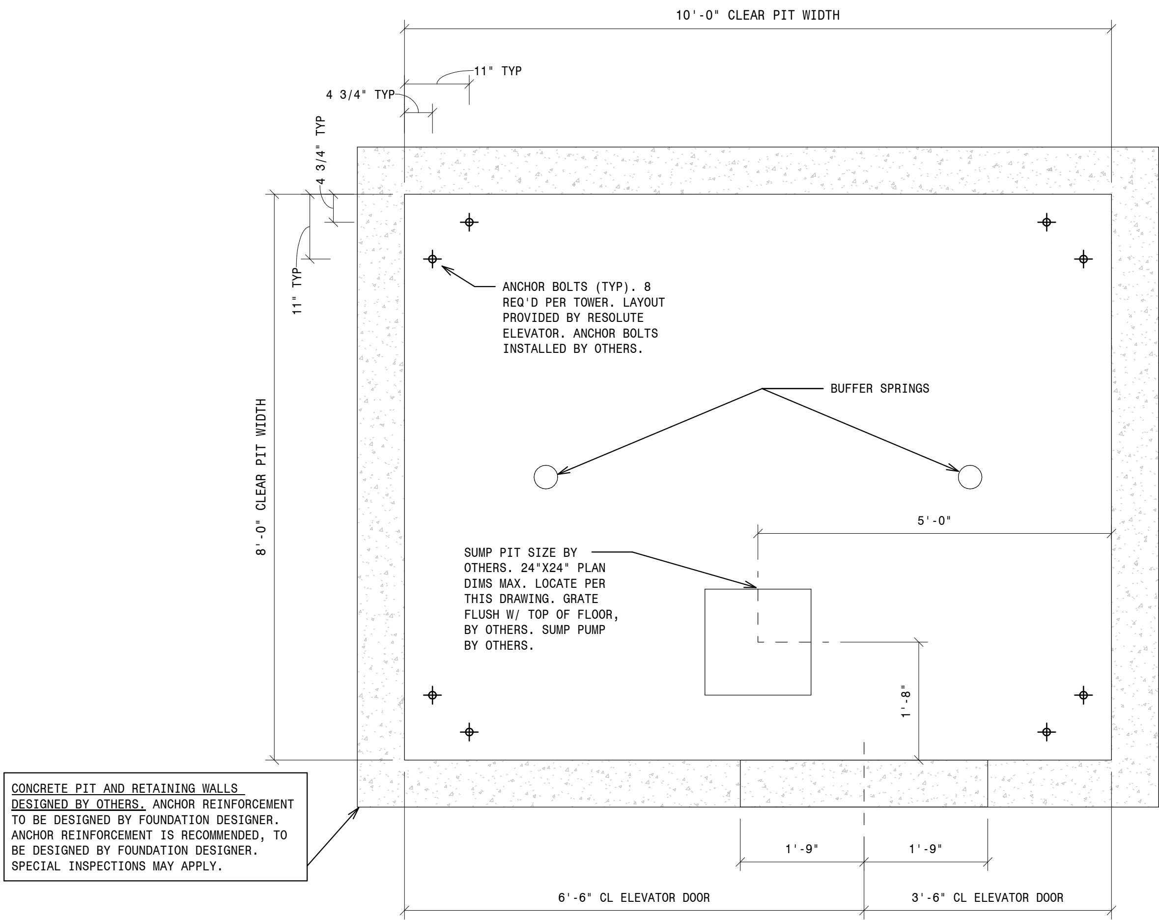
1 - 3500 MRL PIT RIGHT HAND 3/4" = 1'-0"
