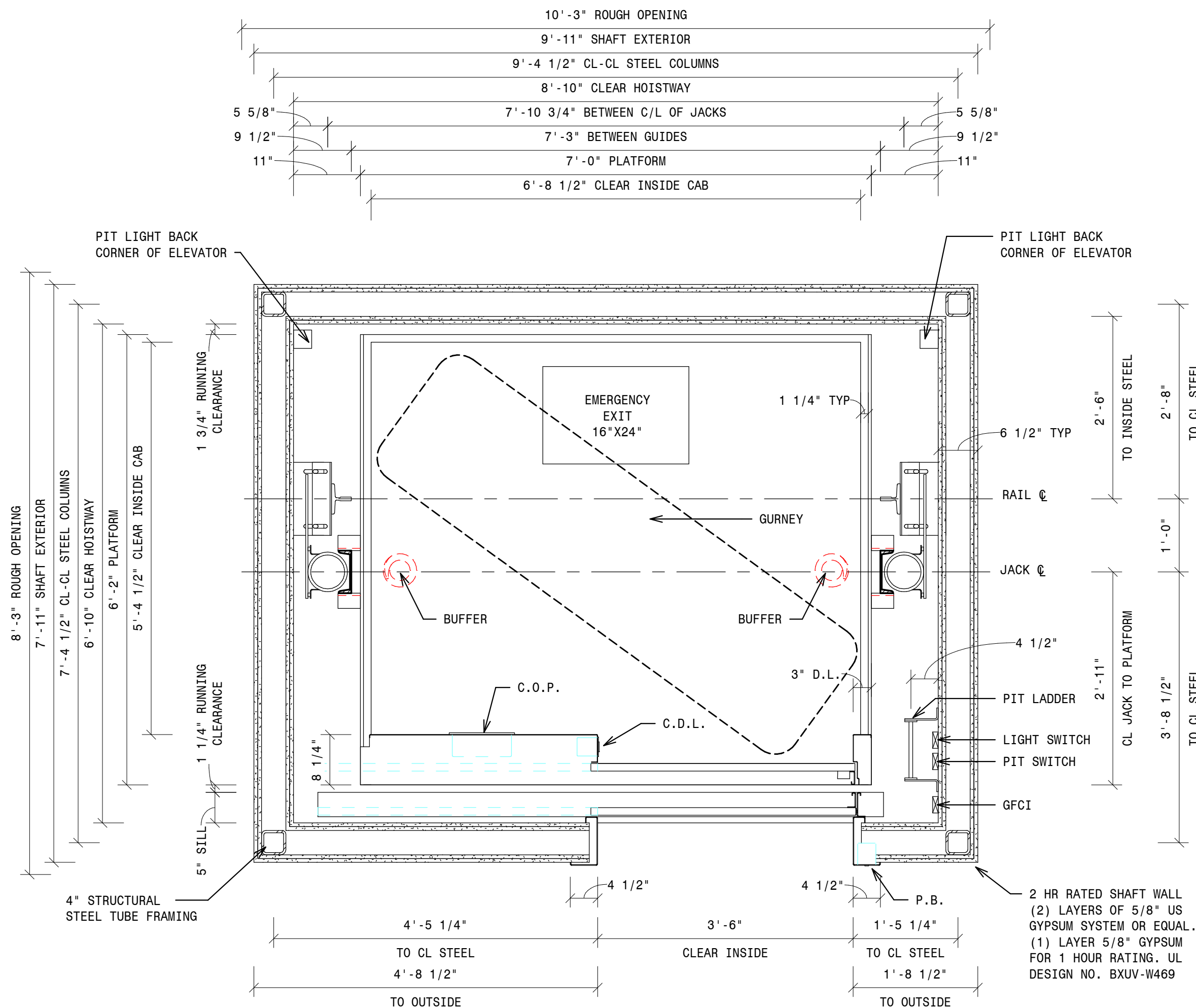
2 - 3500 MRL HOISTWAY RIGHT HAND 3/4" = 1'-0"
