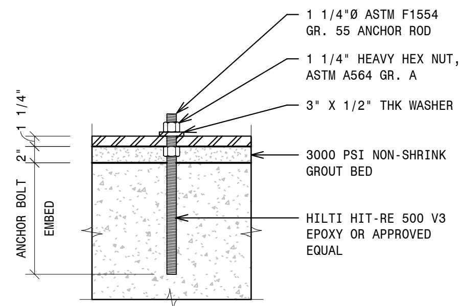
2 - TYPICAL ANCHOR BOLT INSTALLATION NOT TO SCALE
