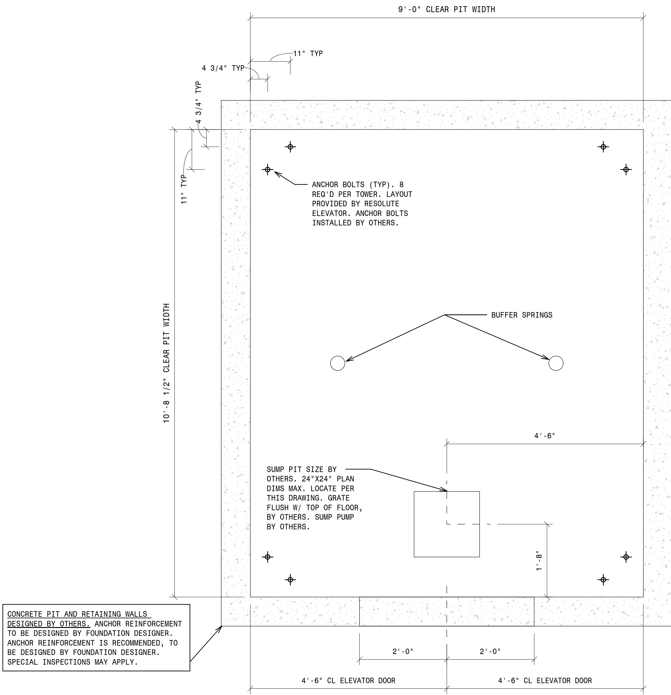
1 - 4500 MRL PIT CENTER 3/4" = 1'-0"
