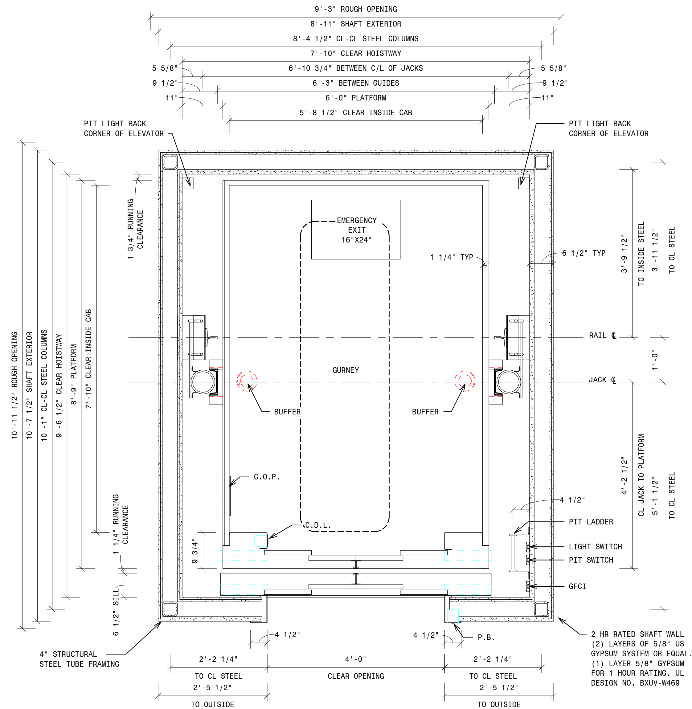
2 - 4500 MRL HOISTWAY CENTER 3/4" = 1'-0"
