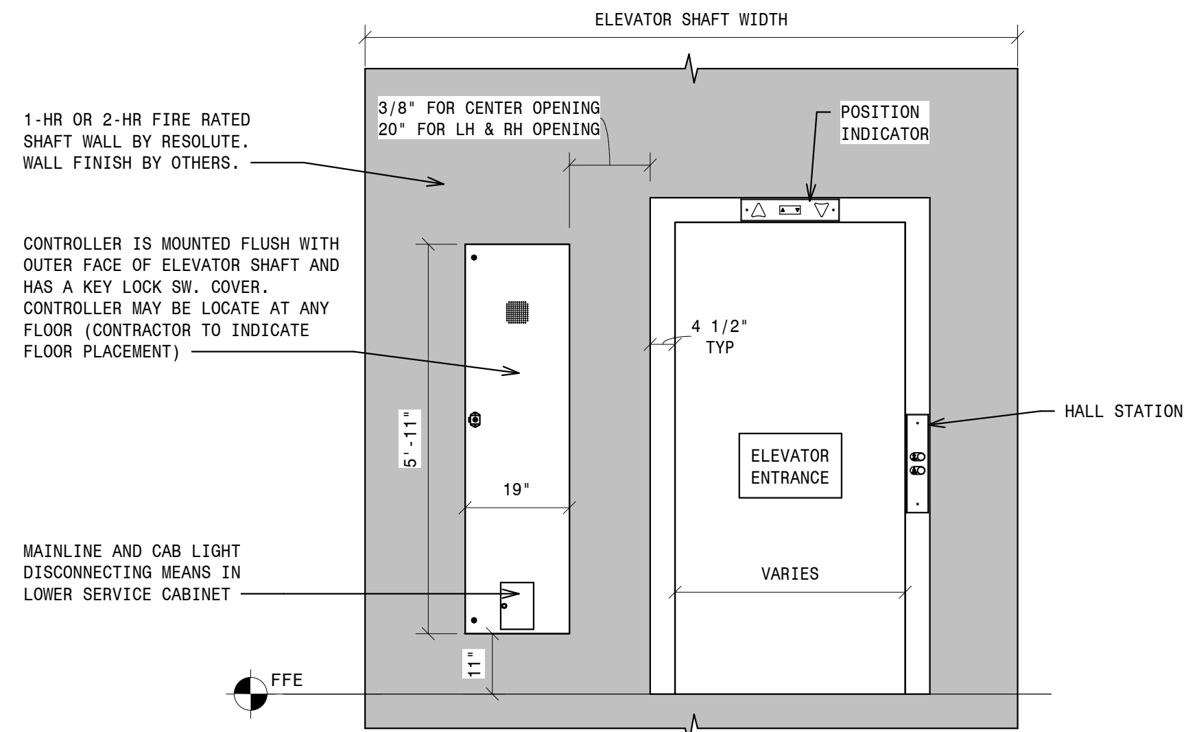
- TYPICAL CONTROLLER LOCATION 1/2" = 1'-0"
