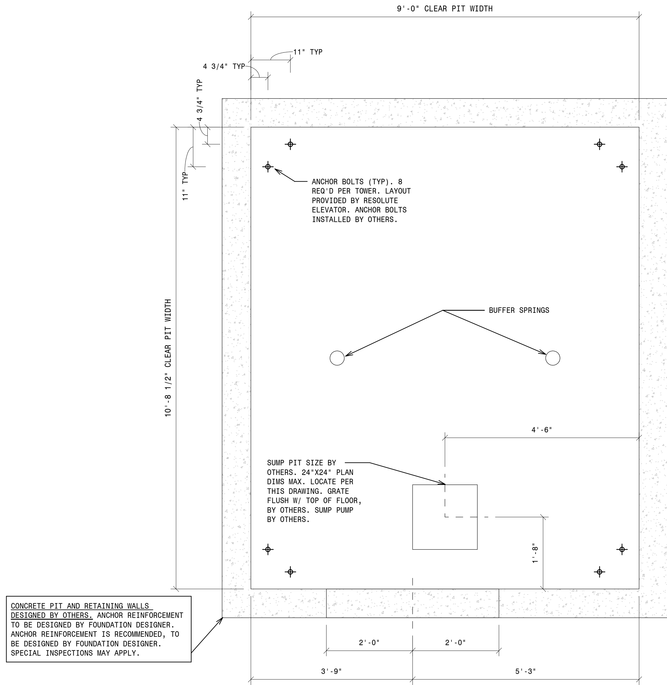
- 1 - 4500 MRL PIT LEFT HAND 3/4" = 1'-0"
