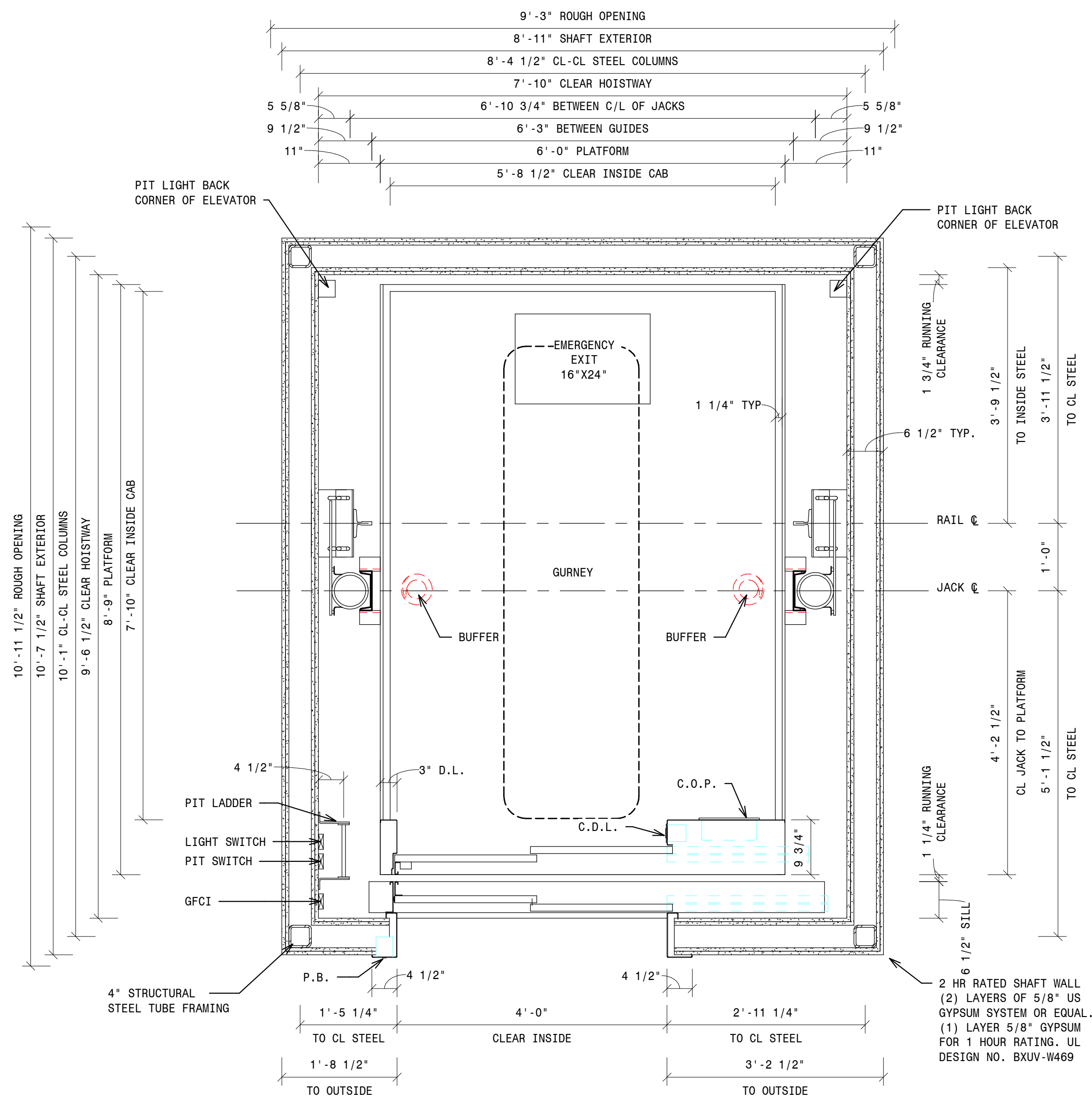
- 2 - 4500 MRL HOISTWAY LEFT HAND 3/4" = 1'-0"
