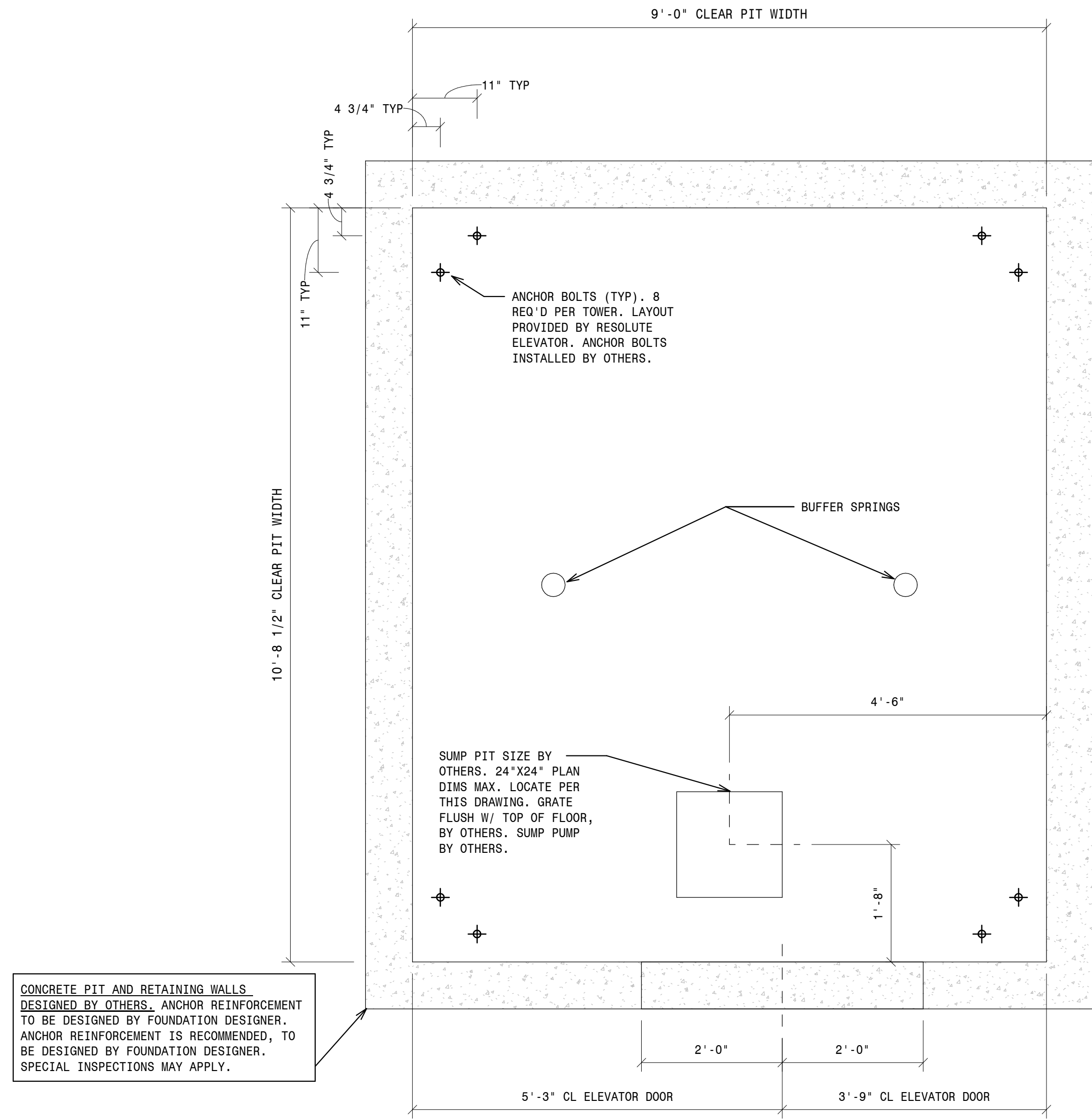
- 1 - 4500 MRL PIT RIGHT HAND 3/4" = 1'-0"
