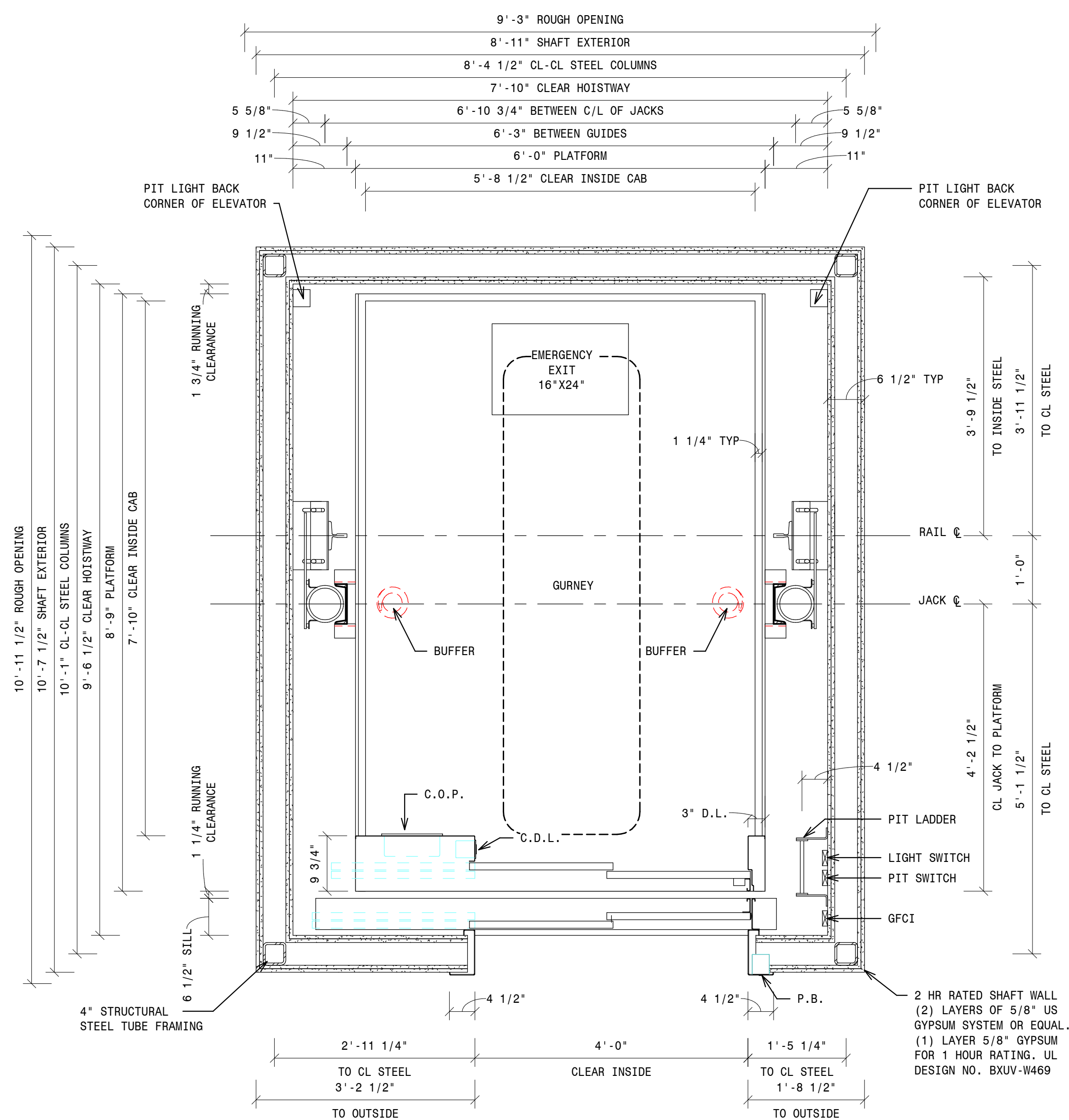
- 2 - 4500 MRL HOISTWAY RIGHT HAND 3/4" = 1'-0"
